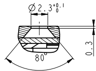
SECTION X-X SCALE 4:1
