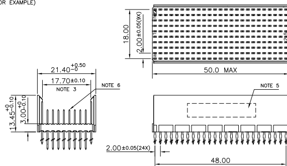
LOADED CONNECTOR ASSEMBLY (FOR EXAMPLE)
