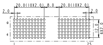
LAY OUT P.C.B -HOLE (FRONT SIDE)
