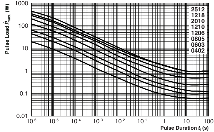
Maximum pulse load, single pulse; applicable if \hat{P} \rightarrow 0 and n < 1000 and \hat{U} \leq \hat{U}_{max} ; for permissible resistance change equivalent to 8000 h operation
