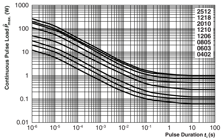
Maximum pulse load, continuous pulses; applicable if \hat{P} \leq P(\vartheta_{amb}) and \hat{U} \leq \hat{U}_{max} ; for permissible resistance change equivalent to 8000 h operation
