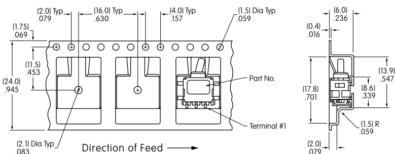
Tape Dimensions
