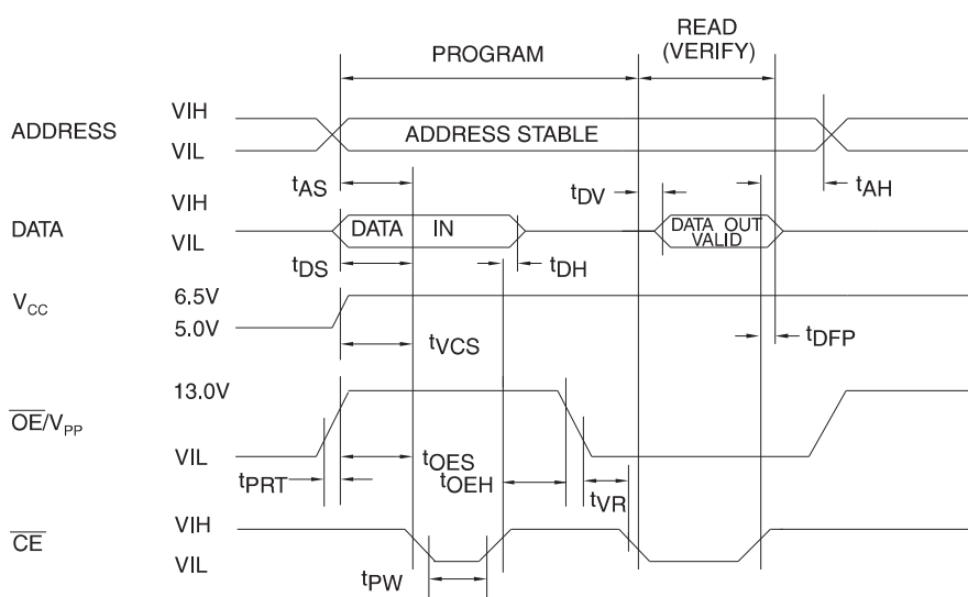
Figure 5-4. Programming Waveforms (1)
