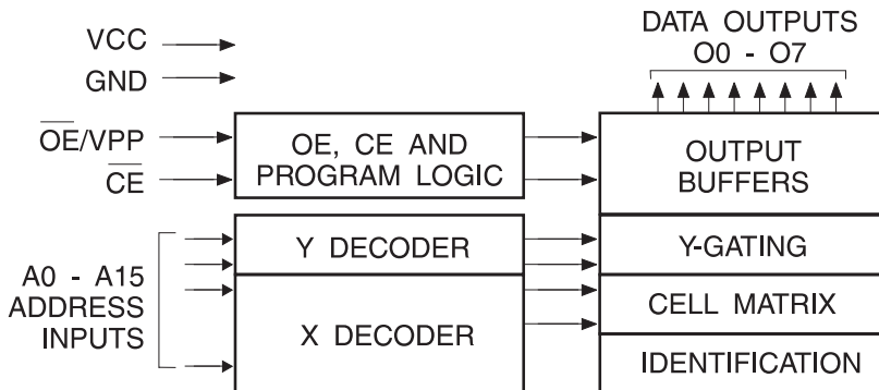
Figure 3-1. Block diagram
