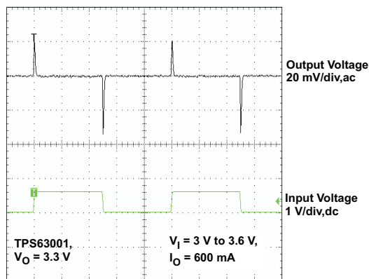
Figure 17. Line Transient Response (TPS63001, I_{OUT} = 600 \text{ mA} )
