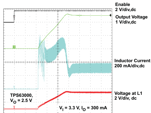
Figure 18. Start-Up After Enable (TPS63000, V_{OUT} = 2.5 \text{ V} )
