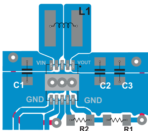
Figure 20. Layout Recommendation
