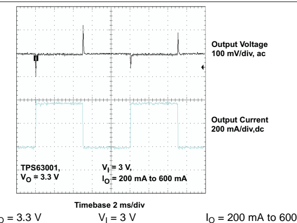
Figure 15. Load Transient Response (TPS63001, V_{IN} < V_{OUT} )
