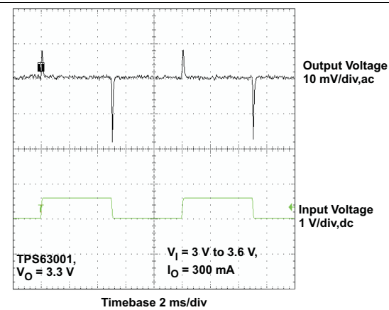
Figure 16. Line Transient Response (TPS63001, I_{OUT} = 300 \text{ mA} )
