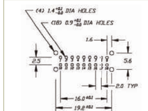
P.C. MOUNTING
