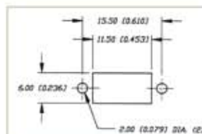
PANEL MOUNT
