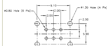
P.C. MOUNTING
