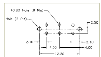
P.C. MOUNTING
