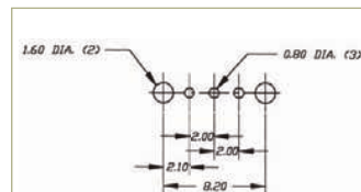
P.C. MOUNTING
