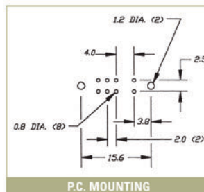
P.C. MOUNTING
