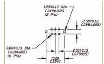
P.C. MOUNTING
