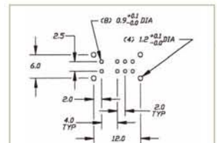
P.C. MOUNTING
