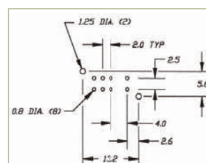
P.C. MOUNTING
