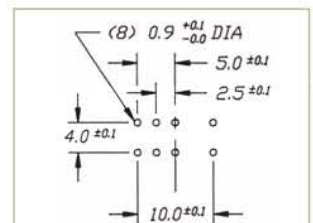
P.C. MOUNTING
