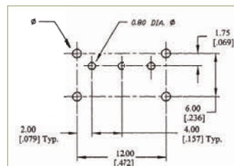
P.C. MOUNTING
