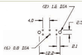
P.C. MOUNTING
