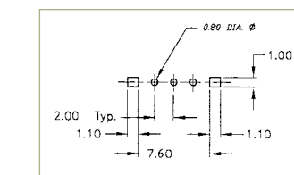
P.C. MOUNTING
