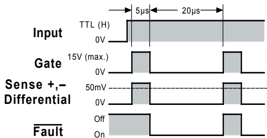
Timing Diagram 2. Fault Condition, C_T = \text{Open}
