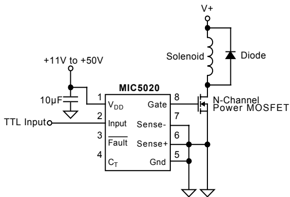
Figure 2. Solenoid Driver, Without Current Sensing
