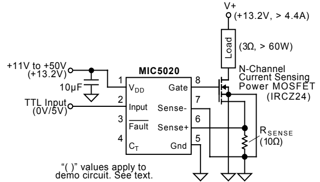
Figure 3. Using a Current Sensing MOSFET
