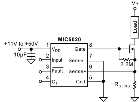
Figure 6a. Gate-to-Source Pull Down
