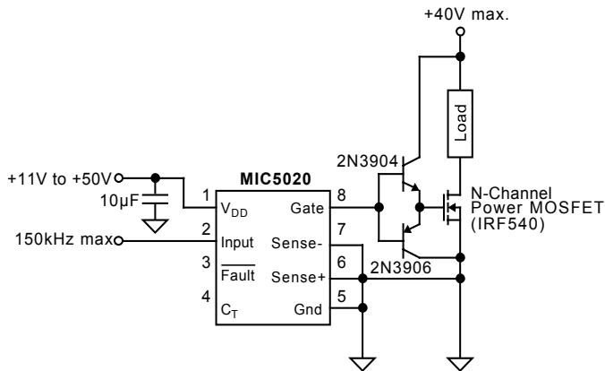
Figure 4. Faster MOSFET Switching Circuit
