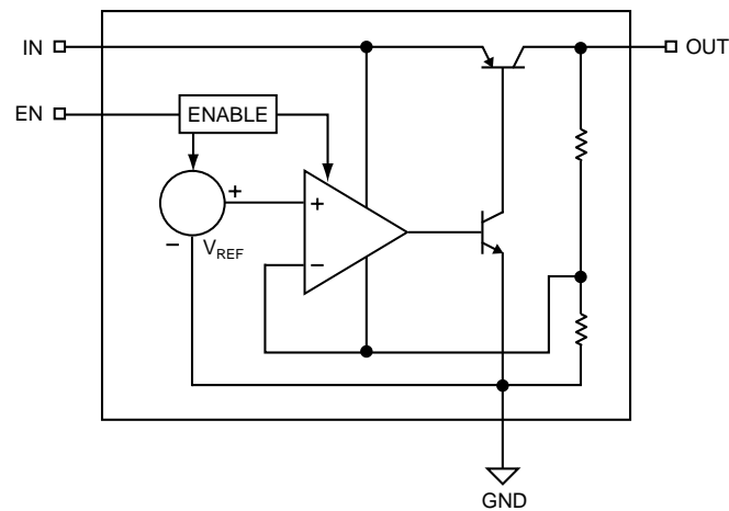
Block Diagram – Fixed Output Voltage
