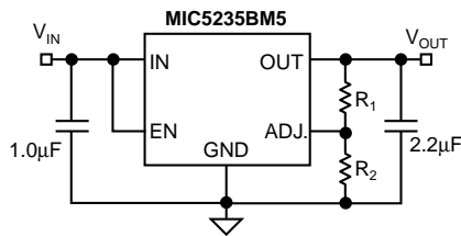
Figure 1. Adjustable Voltage Application
