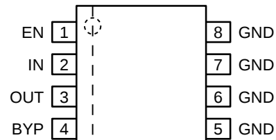
8-Pin MSOP (BMM)
