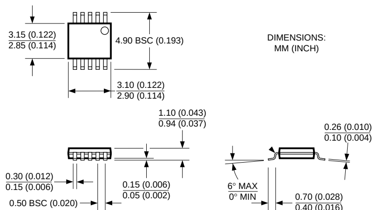
MSOP-10
