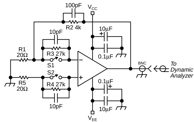
Noise Measurement
