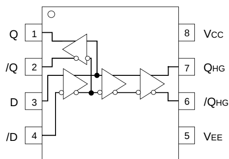
SY10/100EL16VE EL16VB w/Differential Q, QB output (no VBB) (Available in 8-pin SOIC or 8-pin MSOP)
