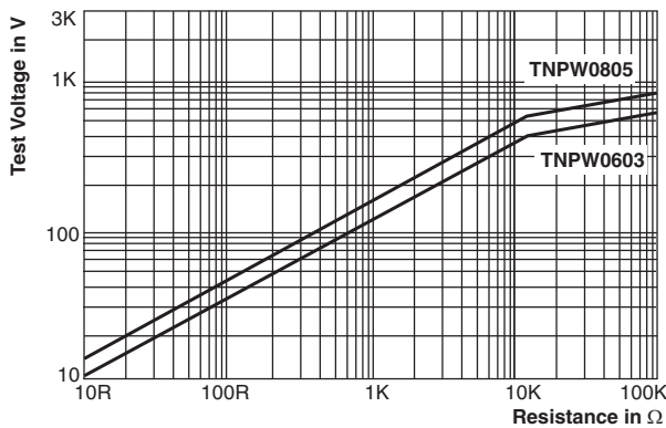
Single-Pulse High Voltage Overload Test 10/700 μs EN 140000 4.27
