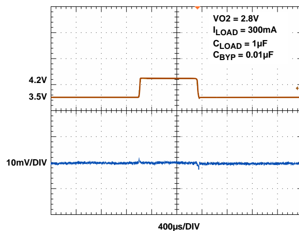
FIGURE 14. LINE TRANSIENT RESPONSE, 2.8V OUTPUT
