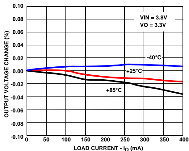
FIGURE 2. OUTPUT VOLTAGE CHANGE vs LOAD CURRENT
