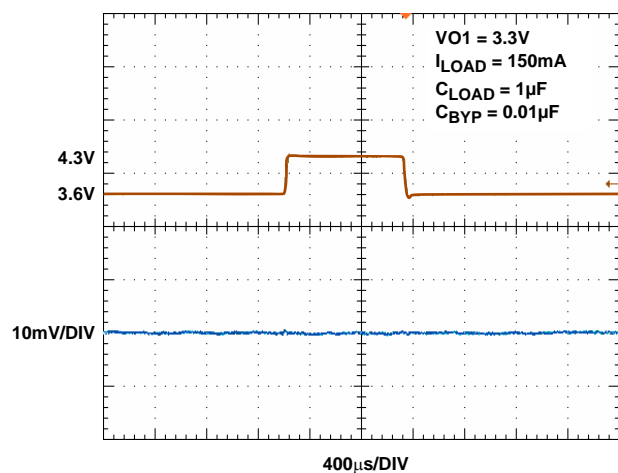
FIGURE 13. LINE TRANSIENT RESPONSE, 3.3V OUTPUT
