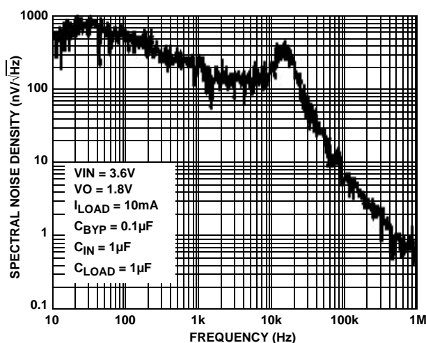
FIGURE 17. SPECTRAL NOISE DENSITY vs FREQUENCY
