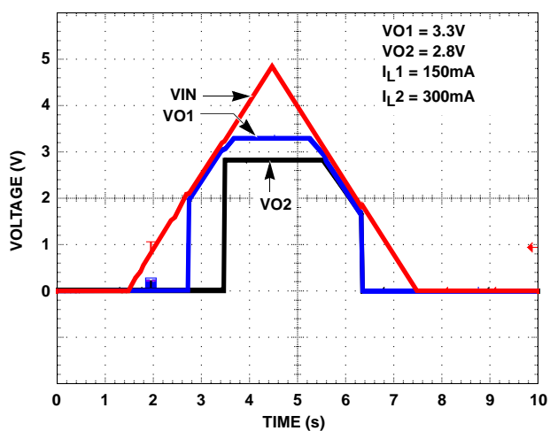
FIGURE 11. POWER-UP/POWER-DOWN
