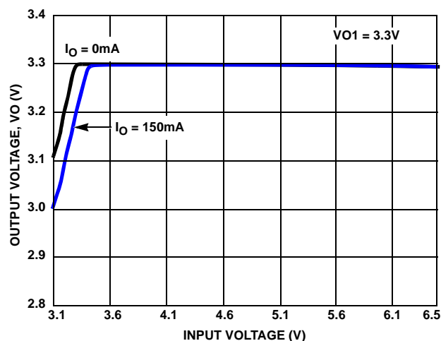
FIGURE 4. OUTPUT VOLTAGE vs INPUT VOLTAGE (VO1 = 3.3V)
