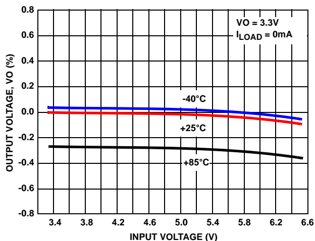
FIGURE 1. OUTPUT VOLTAGE vs INPUT VOLTAGE (3.3V OUTPUT)
