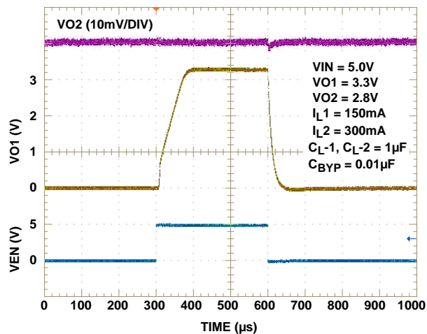
FIGURE 12. TURN-ON/TURN-OFF RESPONSE
