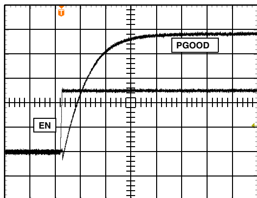
FIGURE 4. EN HIGH to PGOOD
