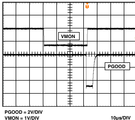
FIGURE 9. VMON LOW to PGOOD
