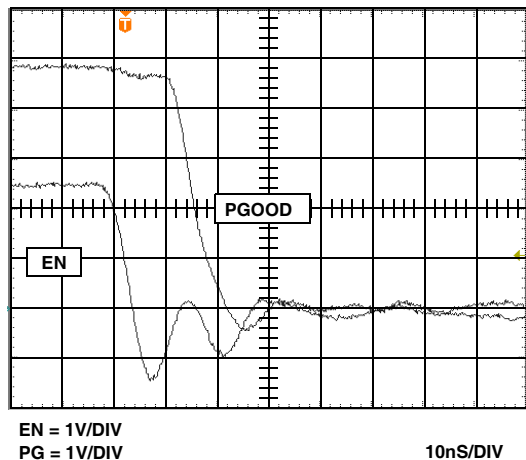
FIGURE 8. EN LOW to PGOOD
