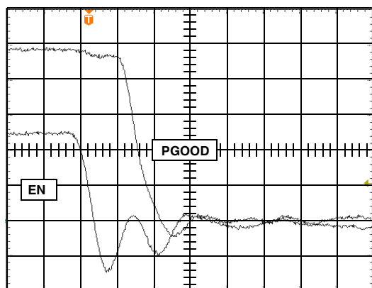
FIGURE 6. EN LOW to PGOOD
