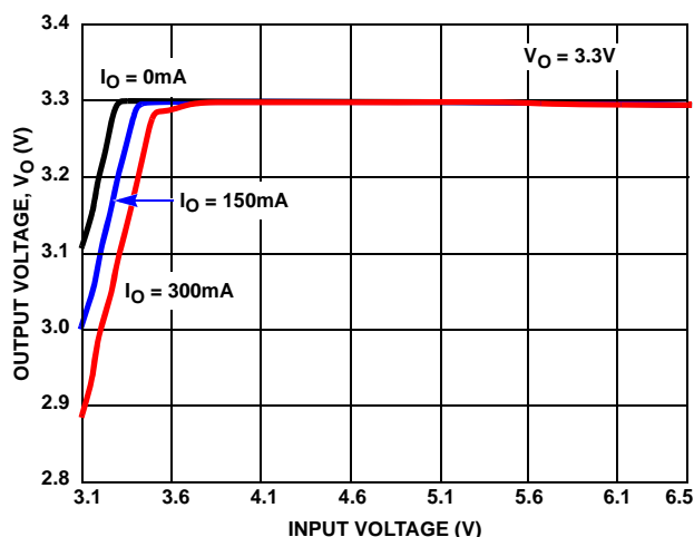
FIGURE 6. OUTPUT VOLTAGE vs INPUT VOLTAGE (3.3V OUTPUT)
