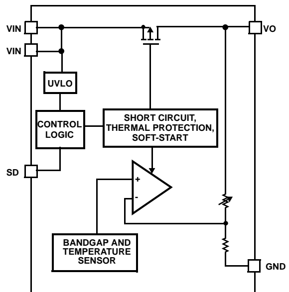
FIGURE 2. BLOCK DIAGRAM
