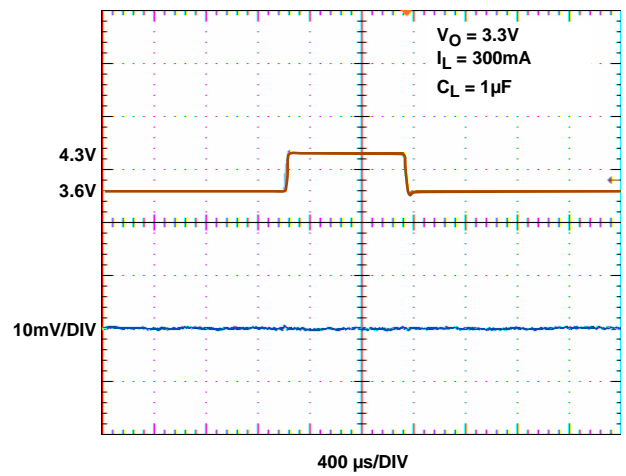
FIGURE 14. LINE TRANSIENT RESPONSE, 3.3V OUTPUT
