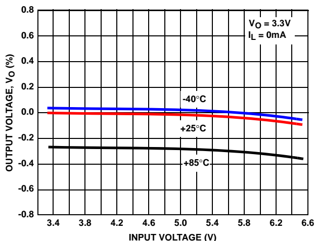
FIGURE 3. OUTPUT VOLTAGE vs INPUT VOLTAGE (3.3V OUTPUT)
