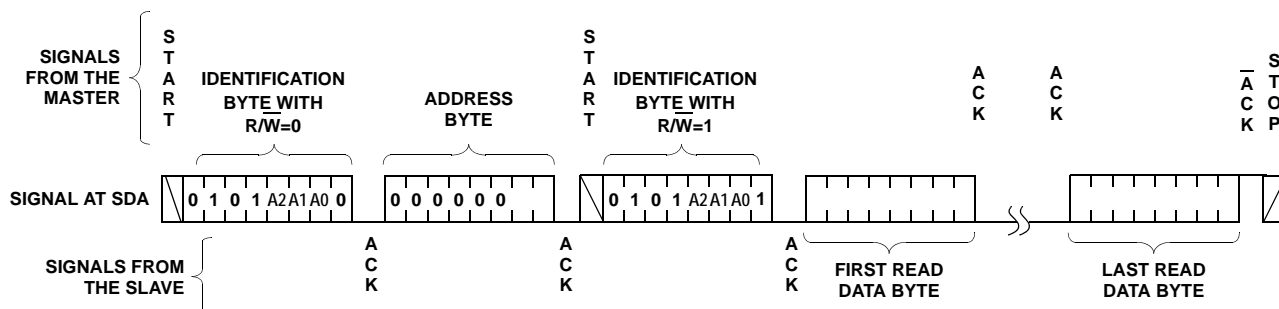
FIGURE 18. READ SEQUENCE
