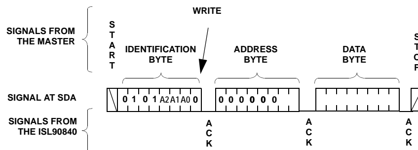
FIGURE 17. BYTE WRITE SEQUENCE
