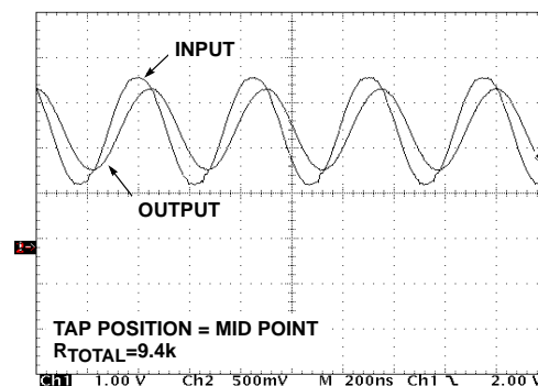
FIGURE 12. FREQUENCY RESPONSE (2.2MHz)
