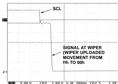
FIGURE 14. LARGE SIGNAL SETTLING TIME
