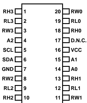
ISL90840 (20 LD TSSOP) TOP VIEW
