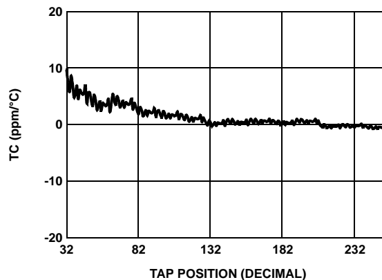
FIGURE 10. TC FOR VOLTAGE DIVIDER MODE IN ppm FOR 50kΩ (W)
