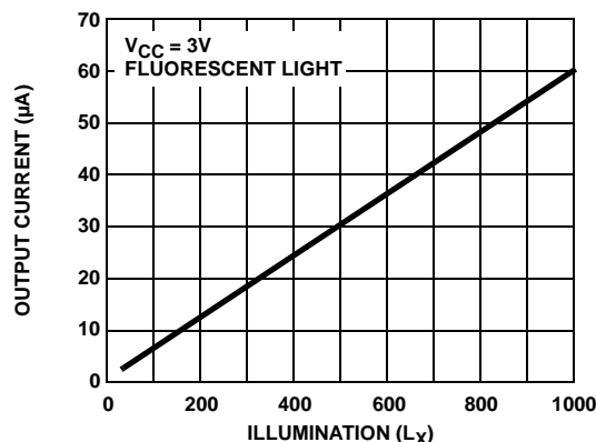
FIGURE 4. SENSITIVITY
