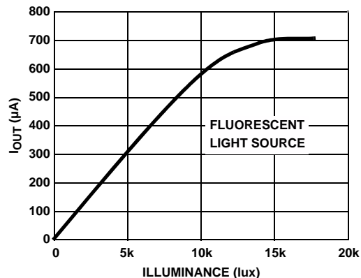
FIGURE 8. I_{OUT} vs LUMINANCE
