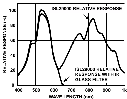
FIGURE 3. SPECTRAL RESPONSE
