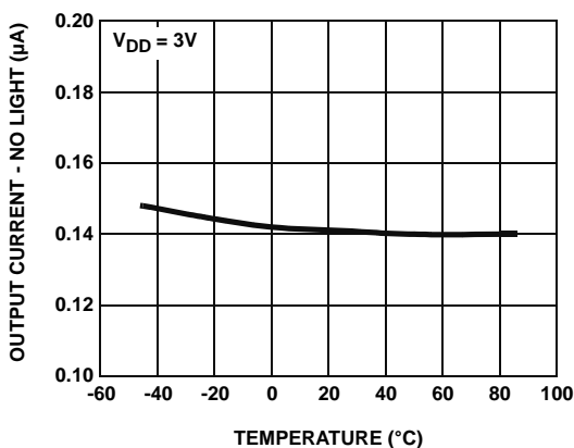
FIGURE 5. DARK CURRENT vs TEMPERATURE
