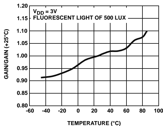
FIGURE 6. GAIN vs TEMPERATURE
