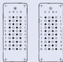
Female insert
