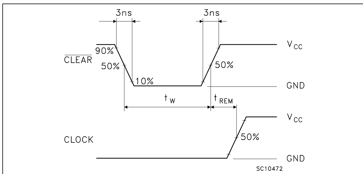
WAVEFORM 3: RECOVERY TIME (f=1MHz; 50% duty cycle)
