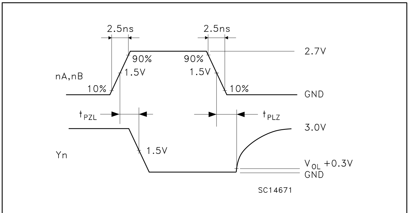
Figure 5: Waveform - Propagation Delays (f=1MHz; 50% duty cycle)
