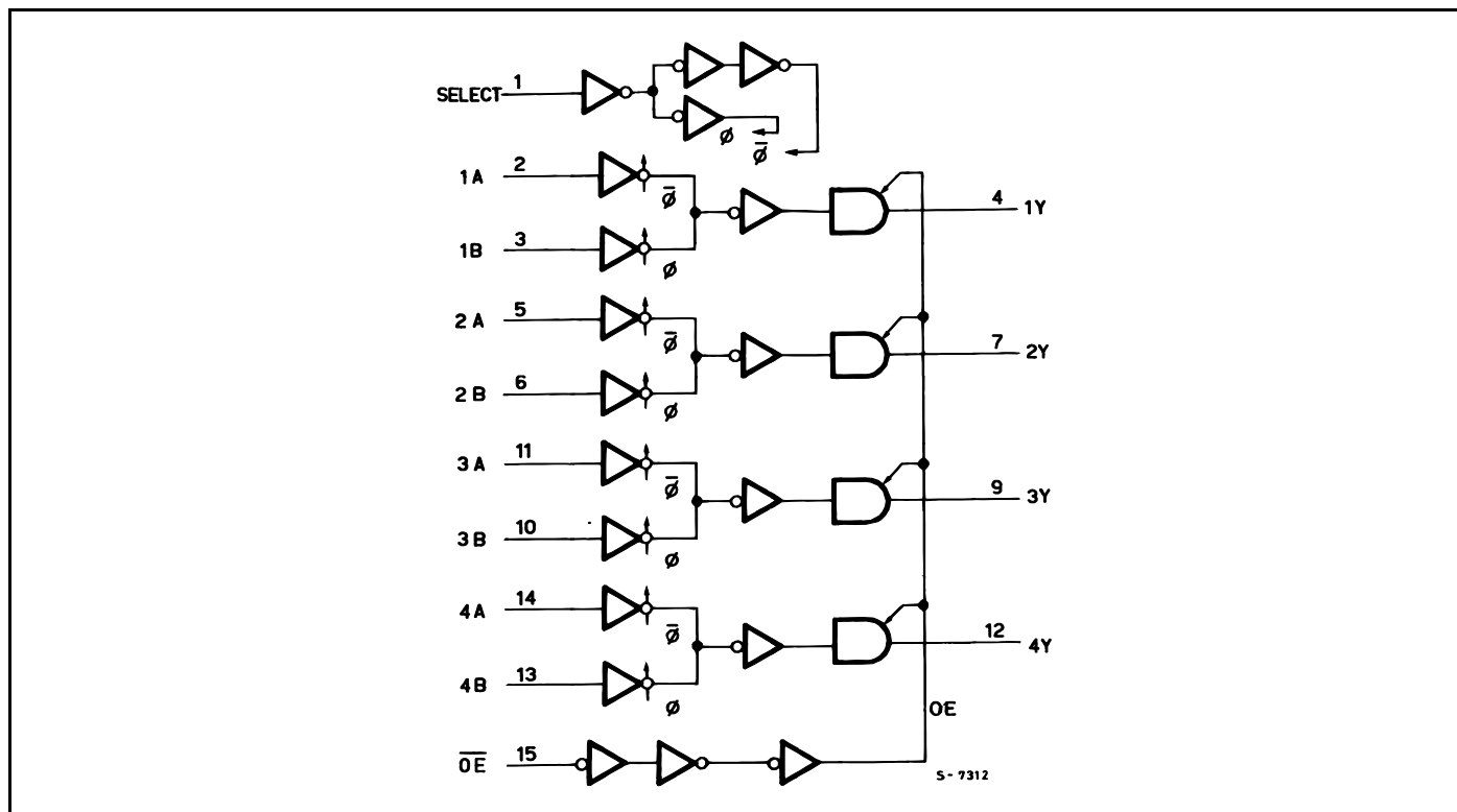
Figure 3: Logic Diagram
