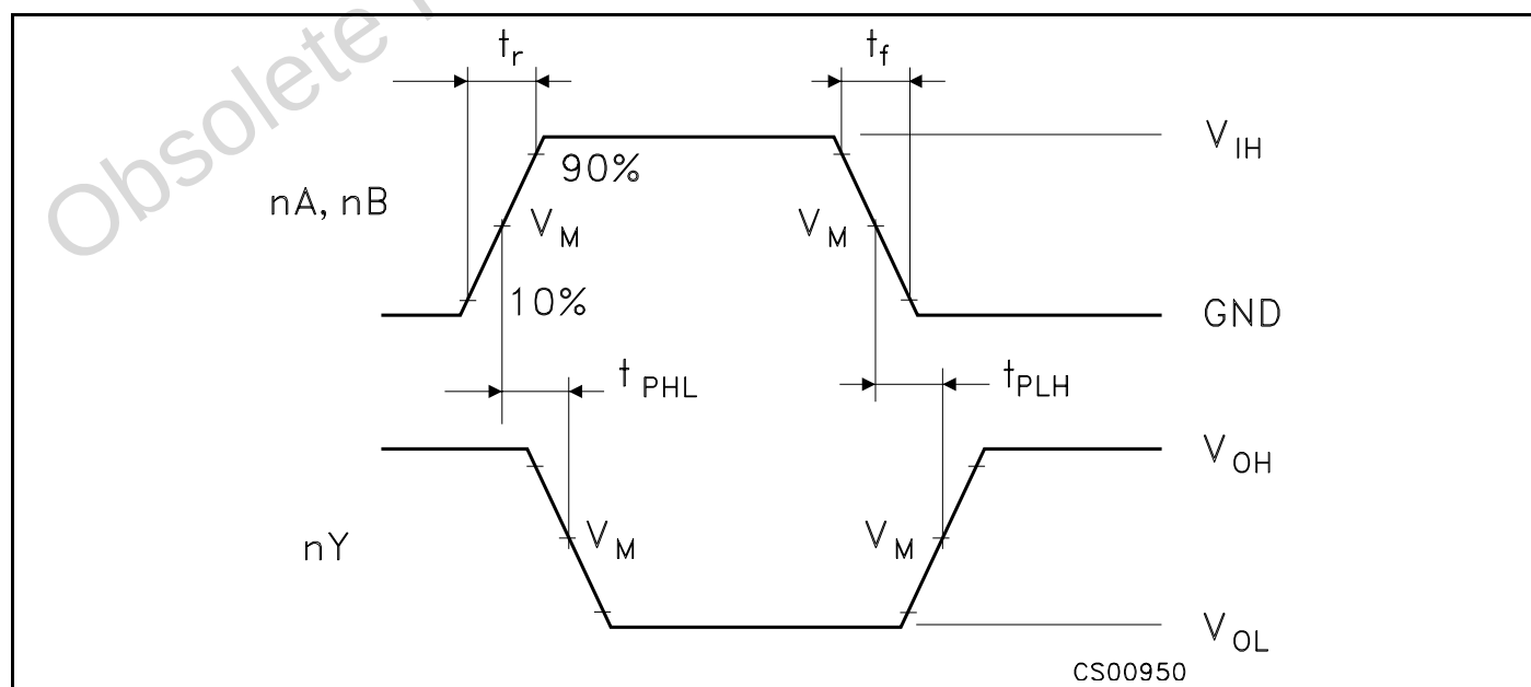
Figure 4: Waveform - Propagation Delay ( f=1\text{MHz} ; 50% duty cycle)
