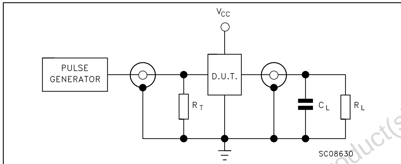
Figure 3: Test Circuit
