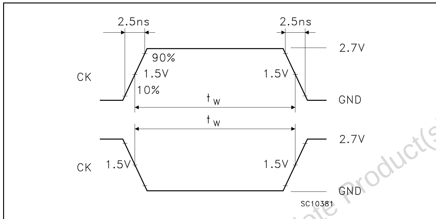
Figure 6: Waveform - Propagation Delay Time ( f=1\text{MHz} ; 50% duty cycle)
