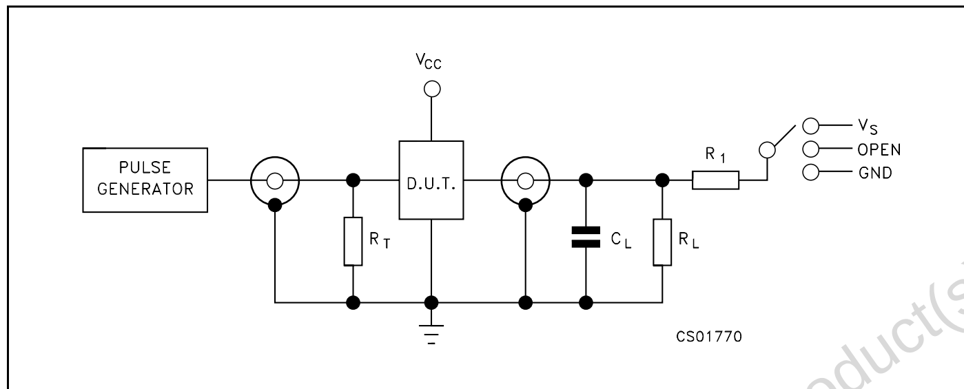
Figure 3: Test Circuit
