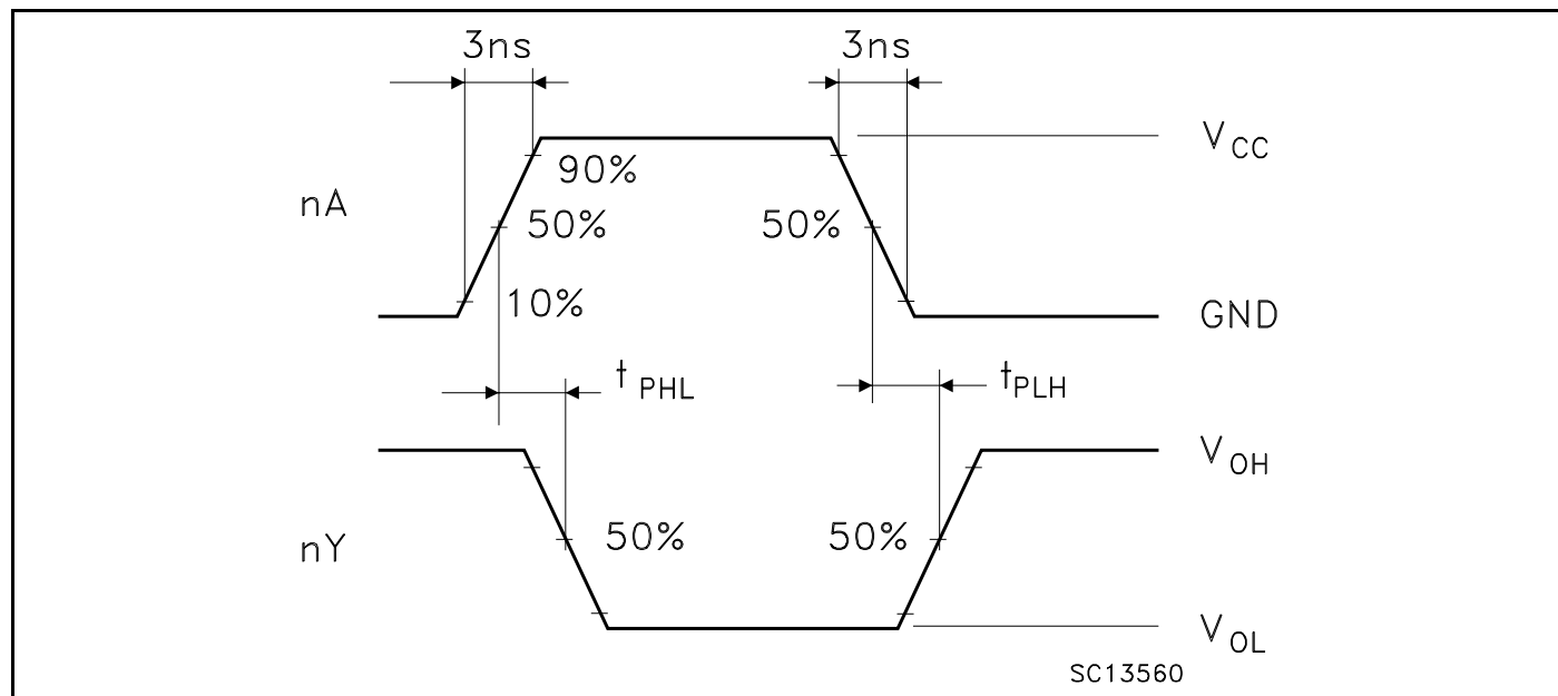
Figure 3: Waveform - Propagation Delays ( f=1\text{MHz} ; 50% duty cycle)
