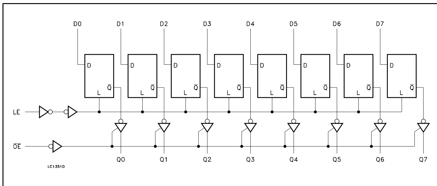
Figure 3: Logic Diagram
