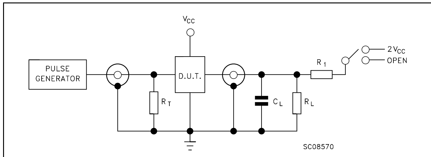
Figure 4: Test Circuit
