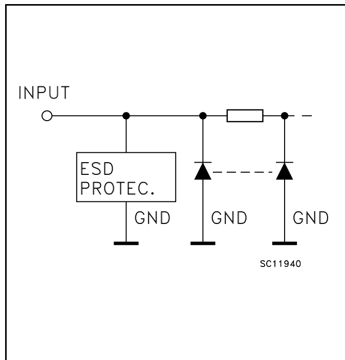
Figure 2: Input Equivalent Circuit
