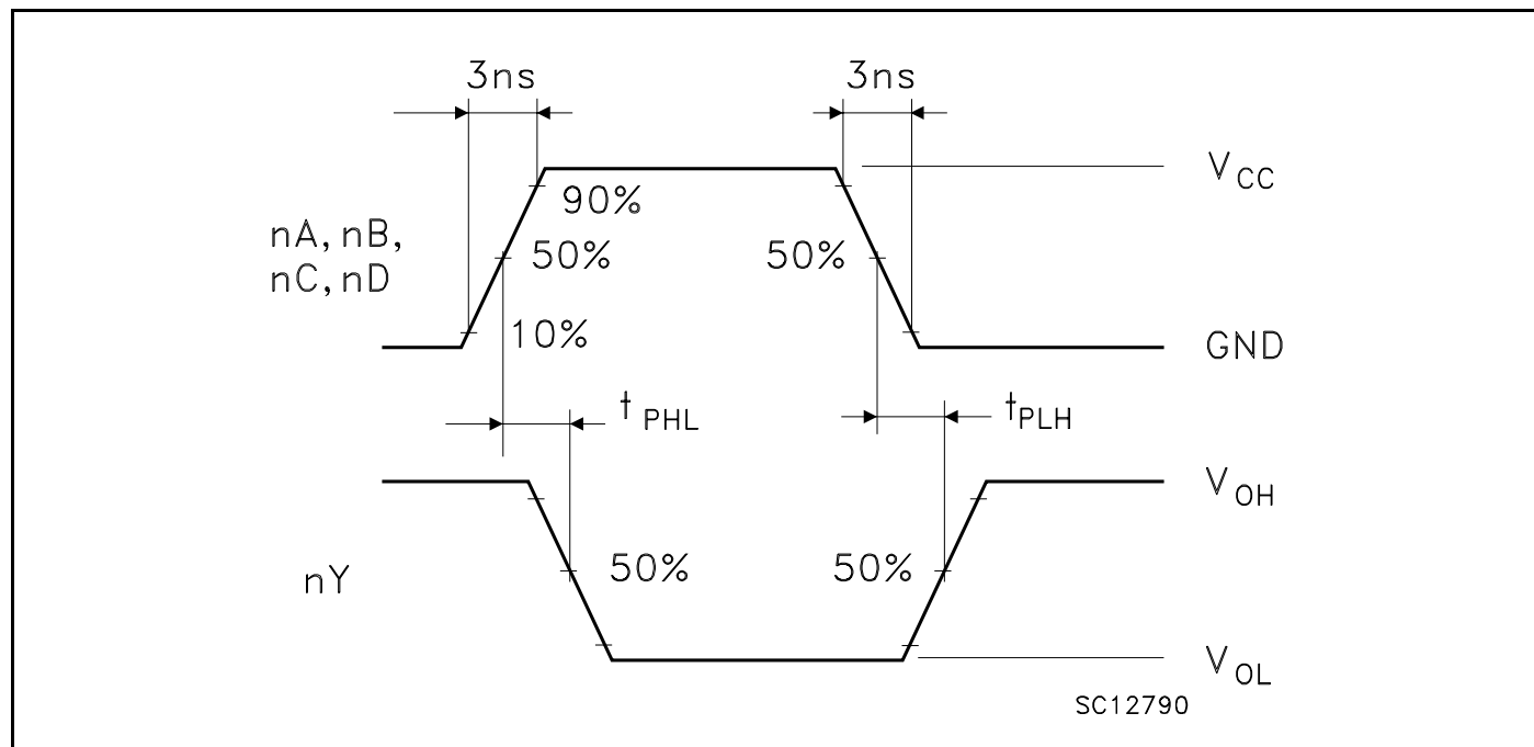
Figure 4: Waveform - Propagation Delays ( f=1\text{MHz} ; 50% duty cycle)
