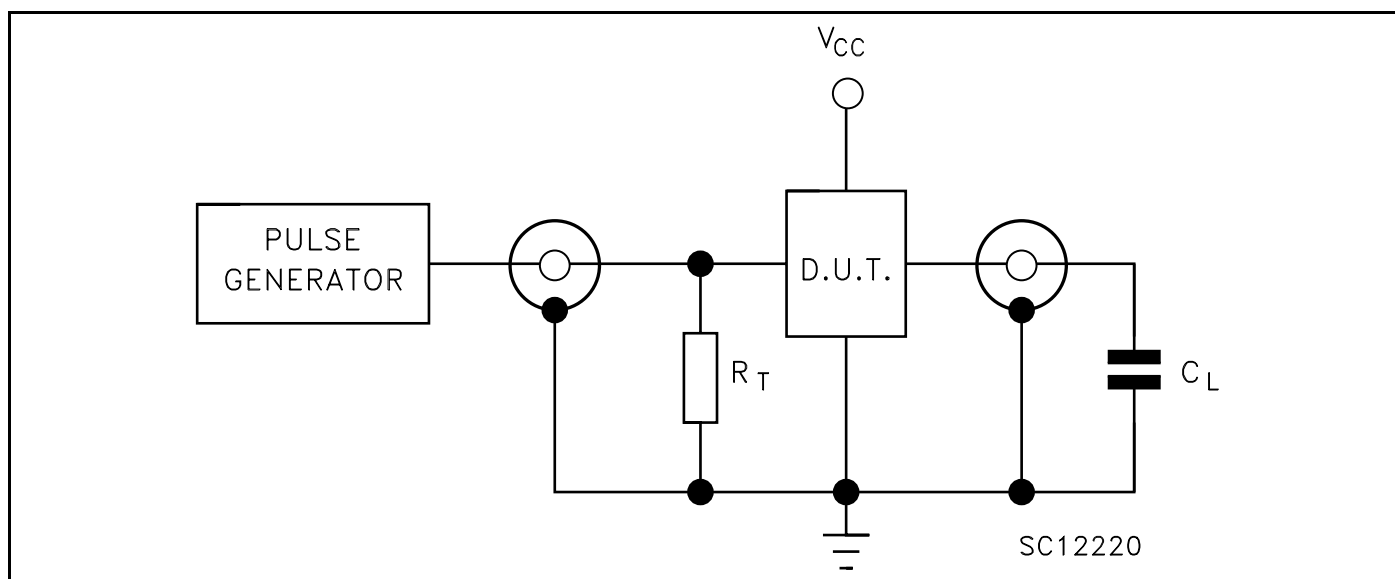
Figure 3: Test Circuit
