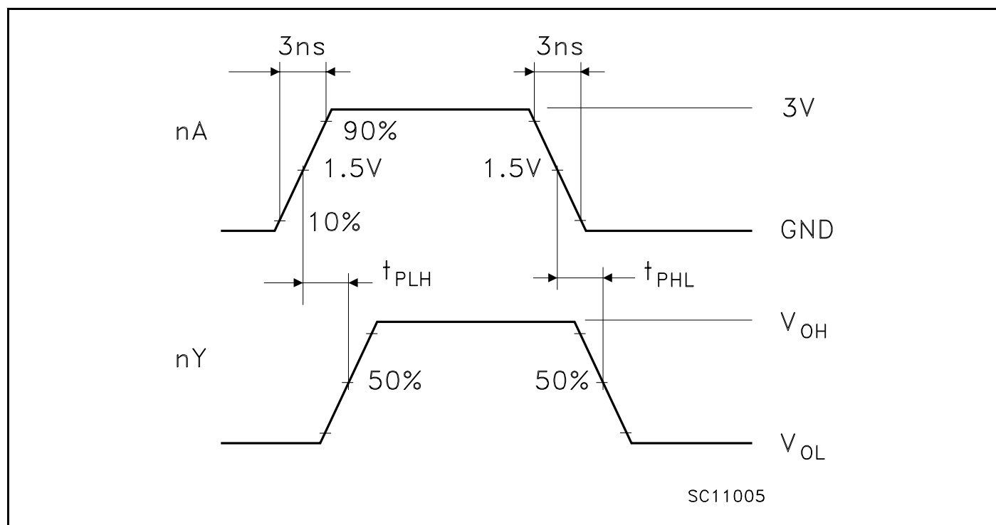
Figure 6: Waveform - Propagation Delays ( f=1\text{MHz} ; 50% duty cycle)
