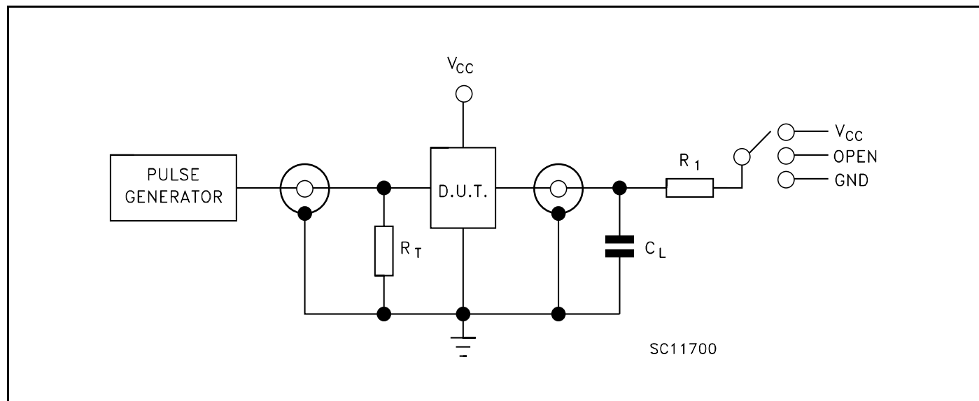
Figure 5: Test Circuit
