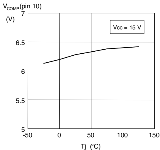
Figure 13. COMP voltage upper clamp level vs. Tj
