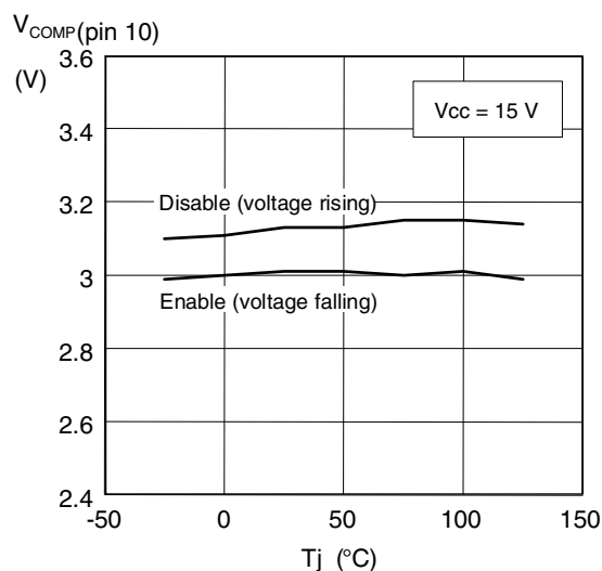
Figure 24. Standby pin dropout vs. Tj
