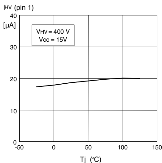
Figure 7. High-voltage pin leakage vs. T_j
