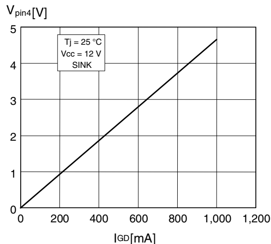
Figure 32. Gate-drive output low saturation
