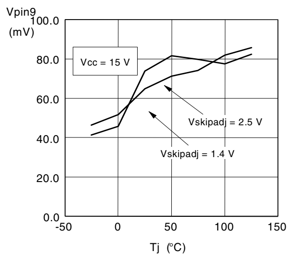
Figure 27. SKIPADJ disable threshold vs. Tj
