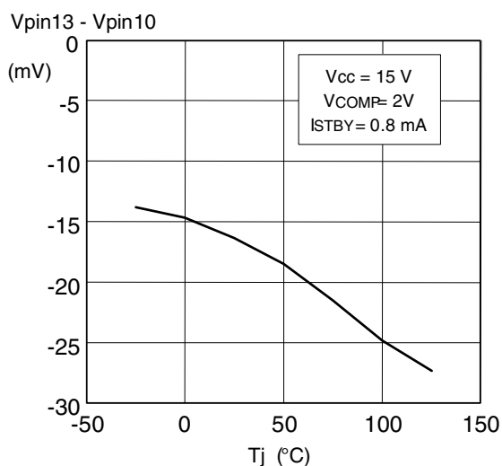
Figure 25. DIS threshold vs. Tj
