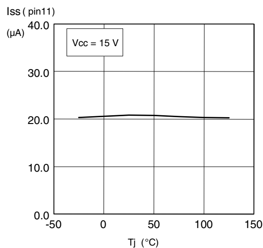
Figure 28. Soft-start charge current vs. Tj
