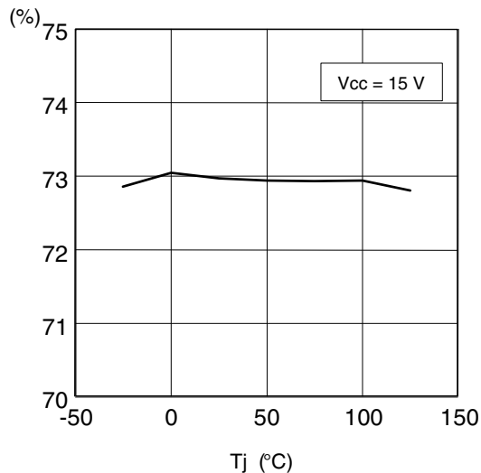
Figure 16. Max. duty-cycle vs. Tj
