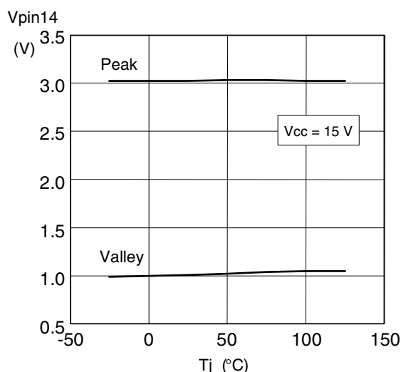
Figure 18. Oscillator ramp vs. Tj
