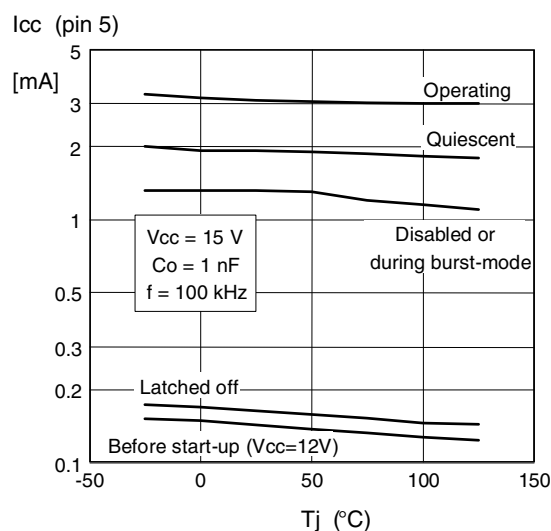
Figure 10. IC consumption vs. T_j
