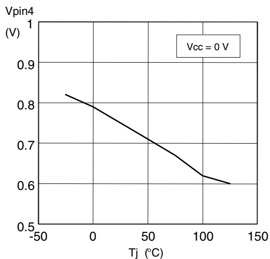
Figure 31. Gate-drive clamp vs. T_j
