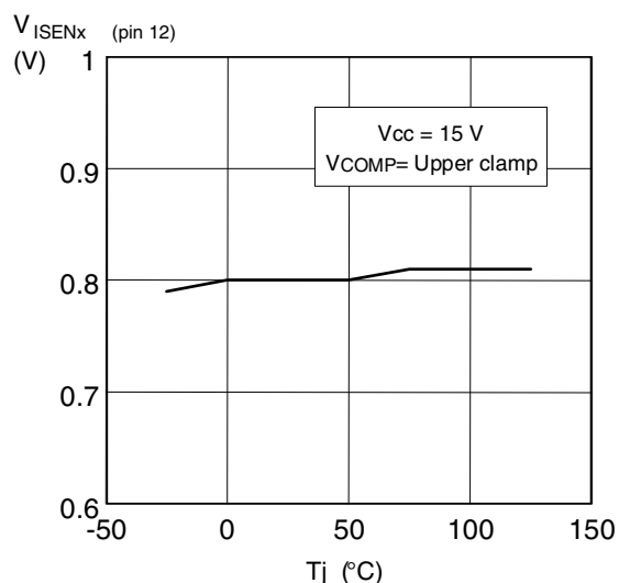
Figure 19. Current sense clamp vs. Tj
