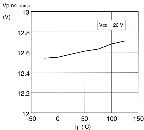
Figure 31. Gate-drive clamp vs. T_j
