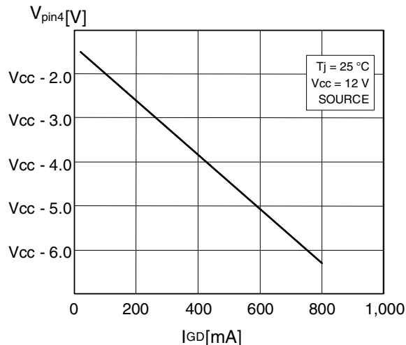
Figure 33. Gate-drive output high saturation
