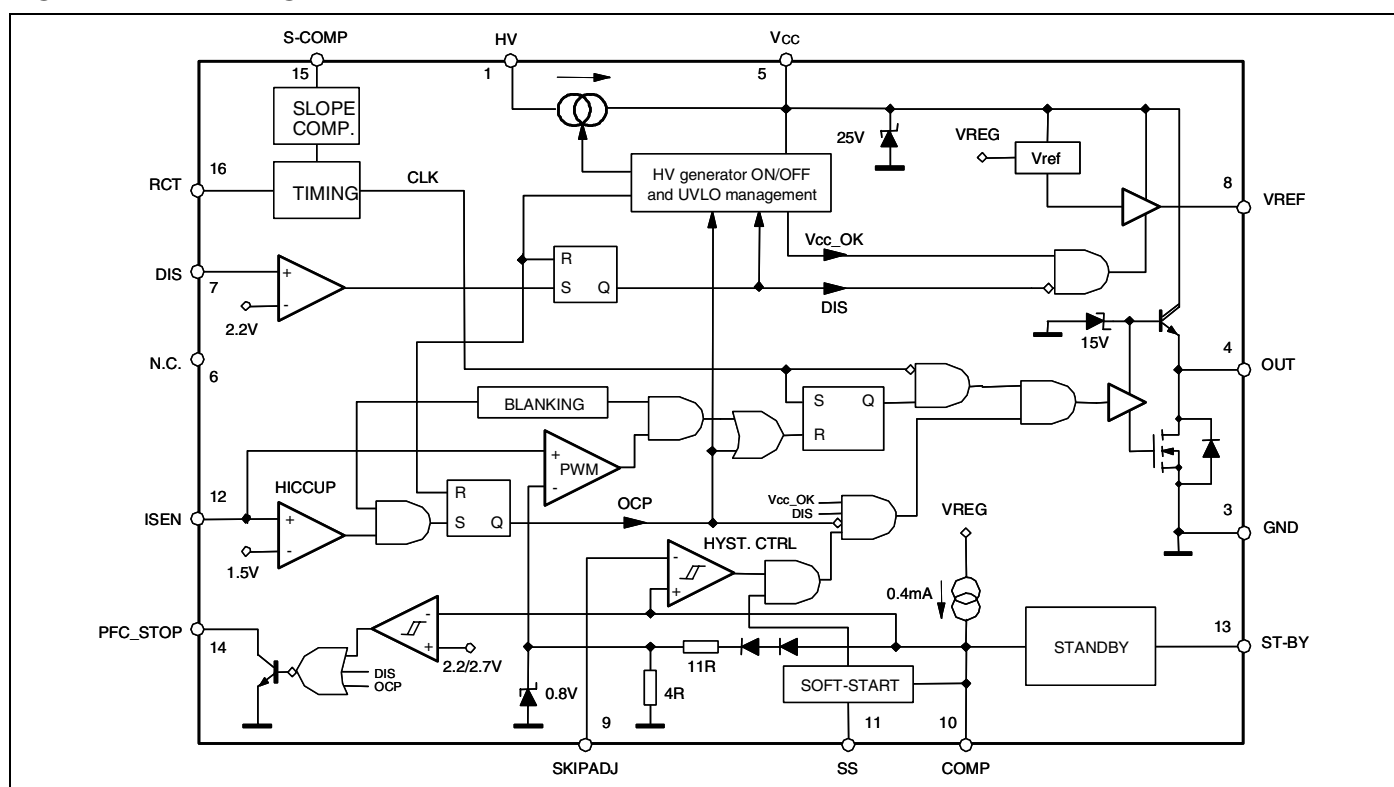
Figure 2. Block Diagram
