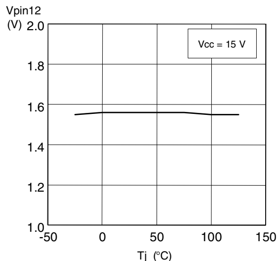
Figure 21. Reference voltage vs. Tj
