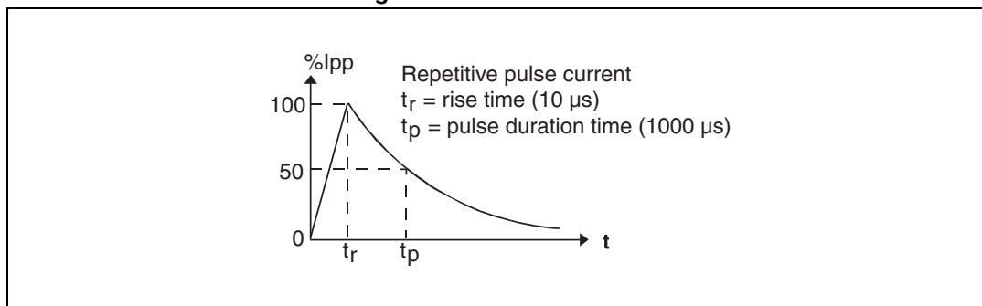
Figure 1. Pulse waveform
