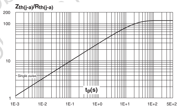
Figure 5: Variation of thermal impedance junction to ambient versus pulse duration (epoxy printed circuit board, e(Cu)=35μm, recommended pad layout)
