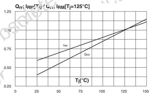
Figure 10: Dynamic parameters versus junction temperature
