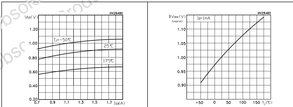
Figure 11. Source-drain diode forward characteristics Figure 12. Normalized B_{V_{DSS}} vs temperature
