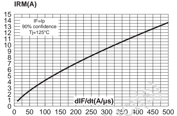
Fig. 6: Reverse recovery current versus dI_F/dt .
