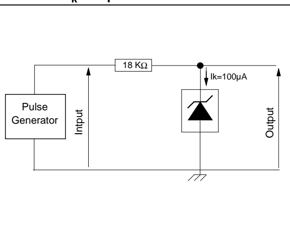
Figure 8. Test circuit for pulse response at I_k=100\mu\text{A}
