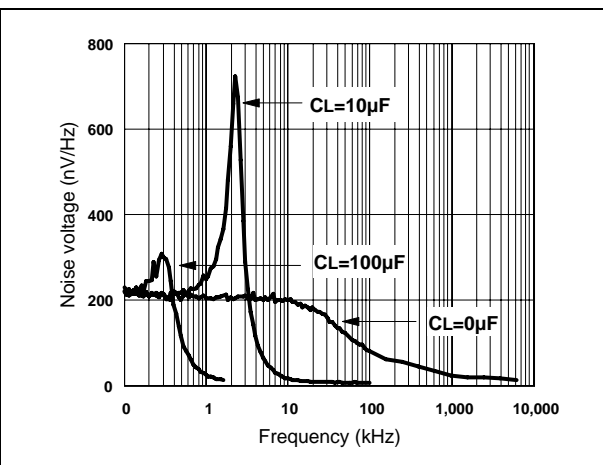
Figure 6. Noise voltage versus frequency
