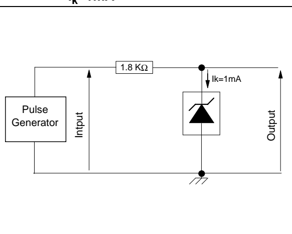
Figure 10. Test circuit for pulse response at I_k=1\text{mA}
