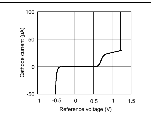
Figure 2. Reference voltage versus cathode current
