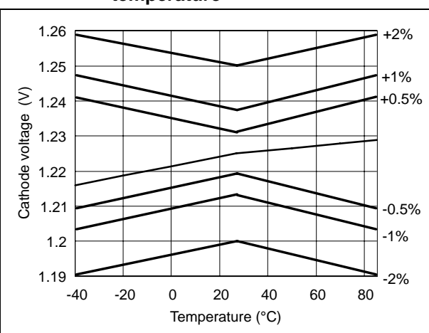
Figure 4. Reference voltage versus temperature
