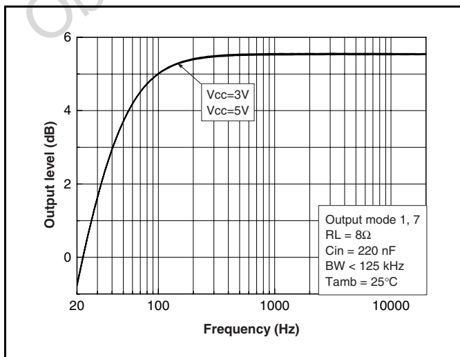
Figure 41: Spkout frequency response (output mode 1, 7)
