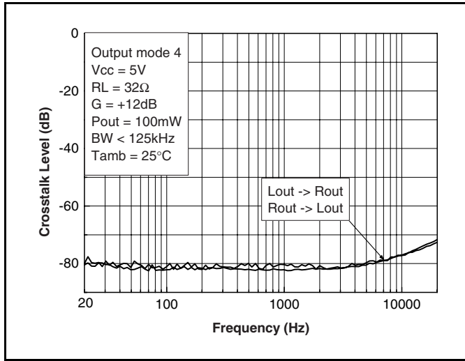
Figure 50: Crosstalk vs. frequency (output mode 4)
