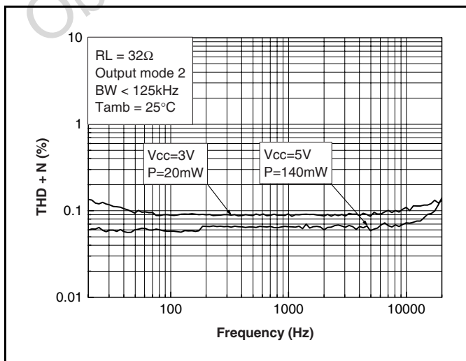
Figure 17: HDout THD+N vs. frequency (output mode 2)
