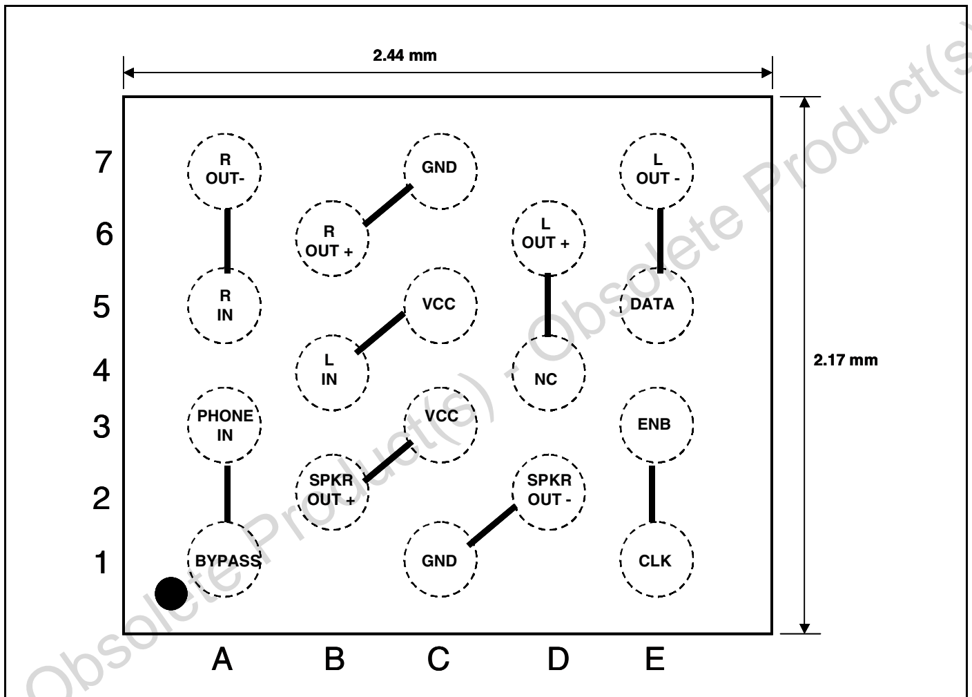
Figure 62: Daisy chain sample mechanical data
