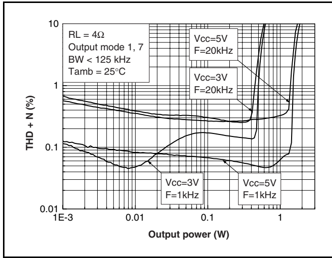
Figure 4: Spkout THD+N vs. output power (output modes 1, 7)
