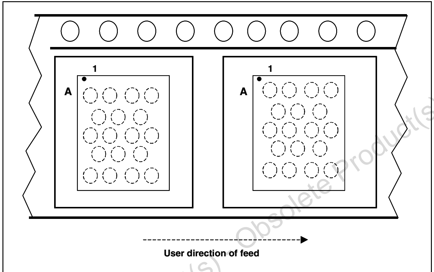
Figure 63: Top view of tape and reel
