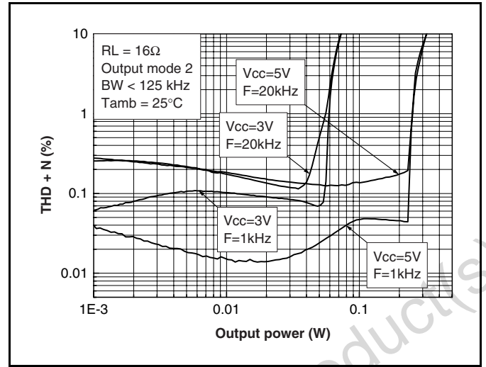
Figure 7: HDout THD+N vs. output power (output mode 2)
