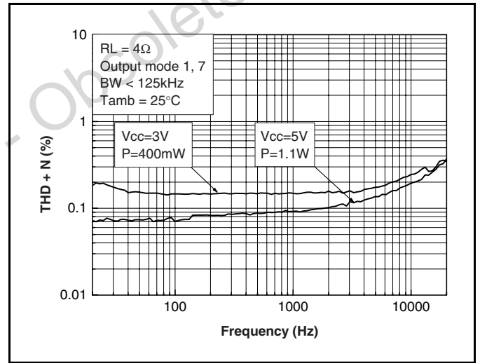
Figure 14: Spkout THD+N vs. frequency (output modes 1, 7)
