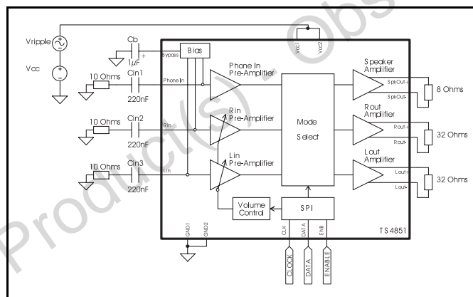
Figure 61: PSRR measurement schematic
