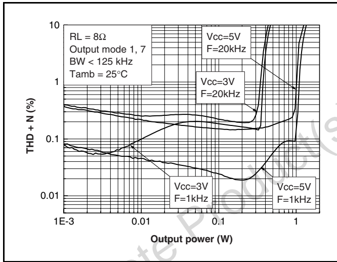
Figure 5: Spkout THD+N vs. output power (output modes 1, 7)
