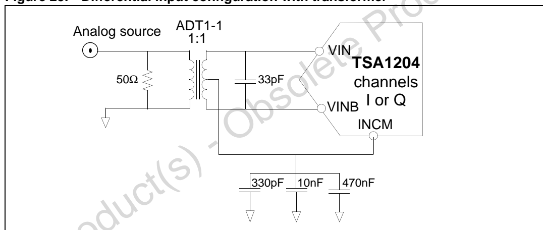
Figure 25. Differential input configuration with transformer
