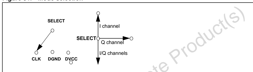
Figure 31. Mode selection
