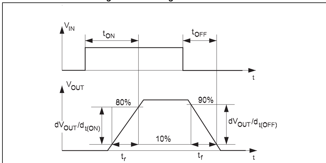
Figure 4. Switching characteristics
