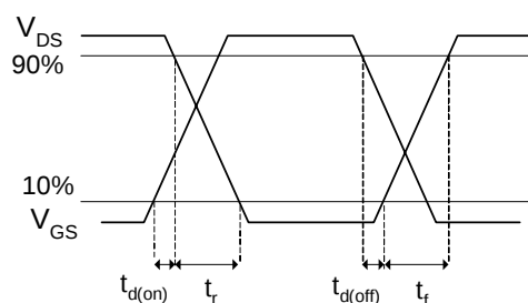
Fig 30b. Switching Time Waveforms
