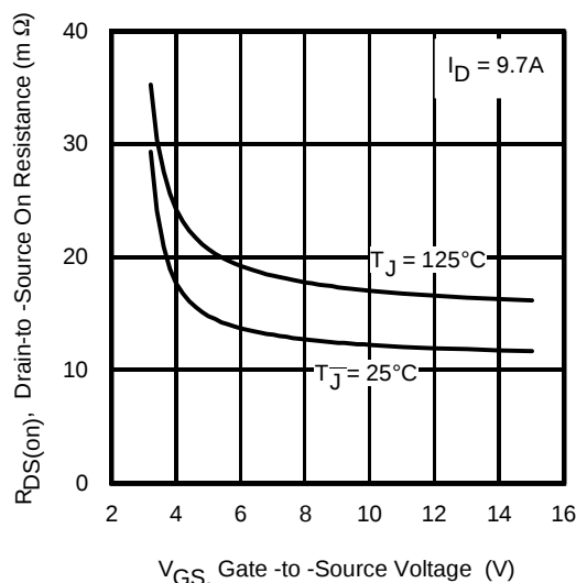
Fig 18. Typical On-Resistance vs. Gate Voltage
