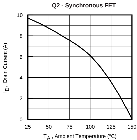
Fig 20. Maximum Drain Current vs. Ambient Temperature
