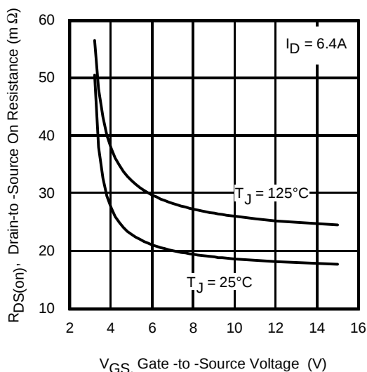
Fig 17. Typical On-Resistance vs. Gate Voltage
