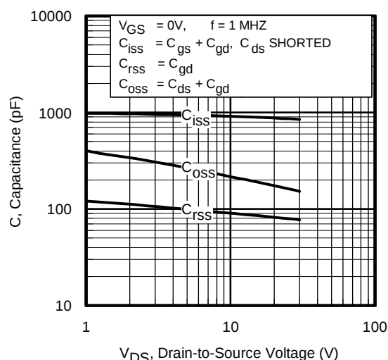
Fig 7. Typical Capacitance vs. Drain-to-Source Voltage Fig 8. Typical Capacitance vs. Drain-to-Source Voltage
