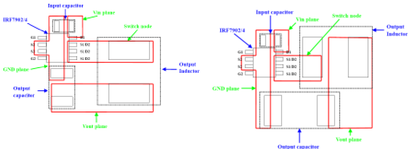
Fig 27. Layout Diagram
