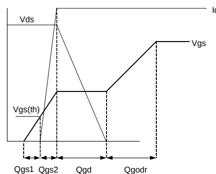
Fig 31b. Gate Charge Waveform
