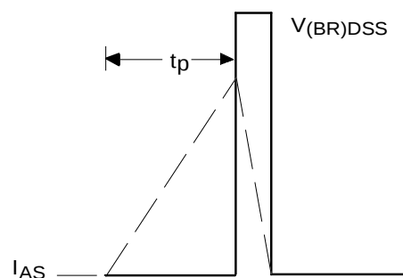
Fig 29b. Unclamped Inductive Waveforms
