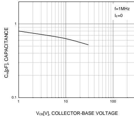
Figure 4. Reverse Capacitance
