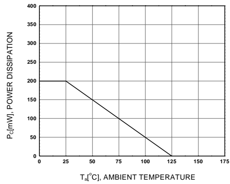
Figure 4. Power Derating
