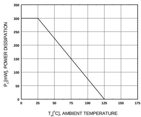
Figure 3. Power Derating
