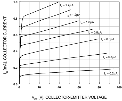
Figure 2. Static Characteristics
