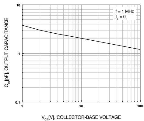
Figure 6. Output Capacitance
