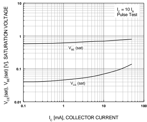
Figure 4. Saturation Voltage
