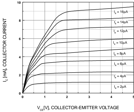
Figure 1. Static Characteristics
