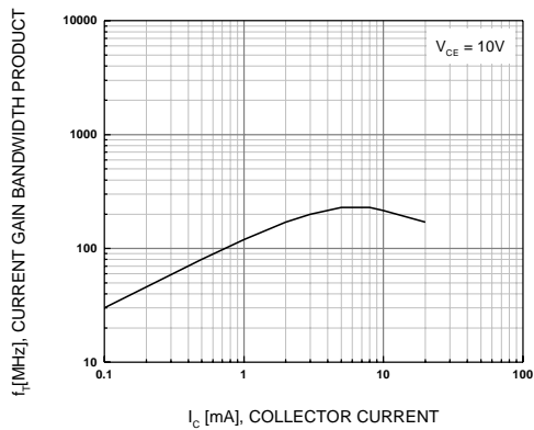
Figure 5. f_T - I_C
