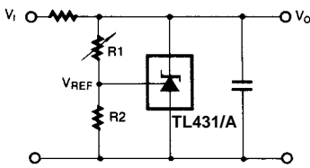
Figure 10. Shunt Regulator
