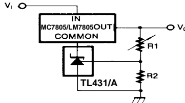
Figure 11. Output Control for Three-Terminal Fixed Regulator
