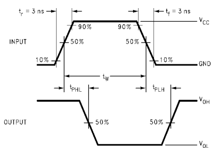
FIGURE 2. AC Waveforms
