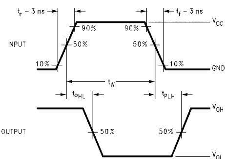
FIGURE 2. AC Waveforms
