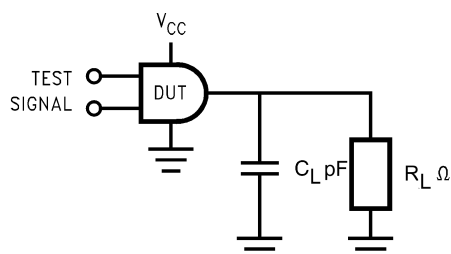
FIGURE 11. AC Test Circuit
