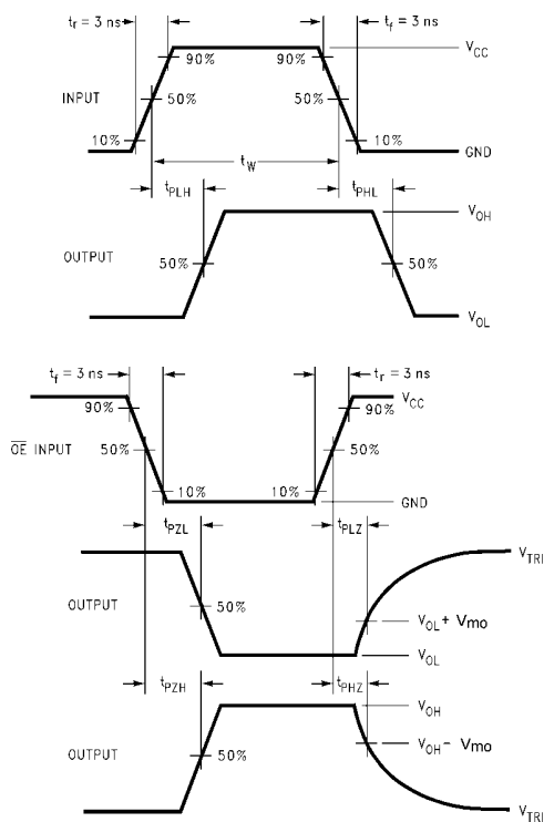
FIGURE 2. AC Waveforms
