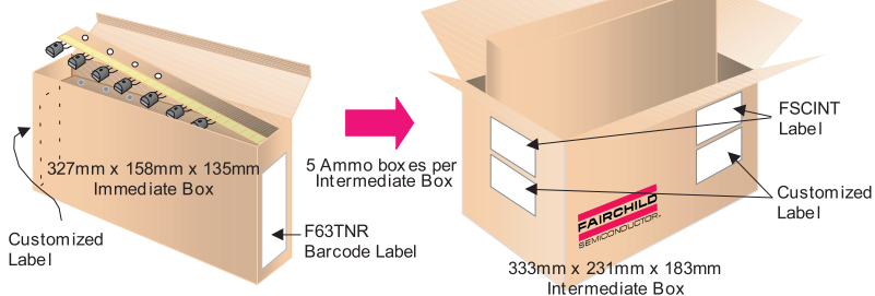
TO-226AE TNR/AMMO PACKING INFORMATION
