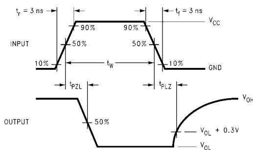
FIGURE 3. AC Waveforms
