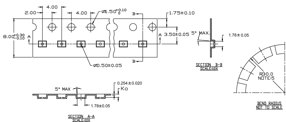
TAPE DIMENSIONS inches (millimeters)
