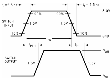
Figure 5. AC Waveform
