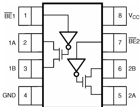
Figure 2. TSSOP Pin Outs (Top View)
