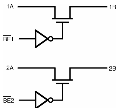
Figure 1. Logical Connections for the FSTD3306
