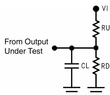
Figure 4. AC Test Circuit. Input driven by 50Ω source-terminated in 50Ω. C_L includes load and stray capacitance. Input PRR = 1.0 MHz; T_w = 500ns.
